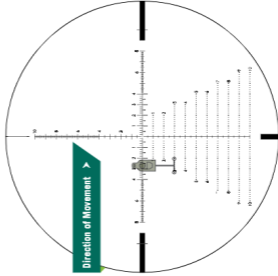
2.7 MRAD correction for a target moving 3 mph.
