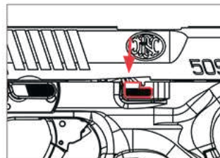
Slide released.
