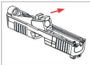
Remove barrel.
