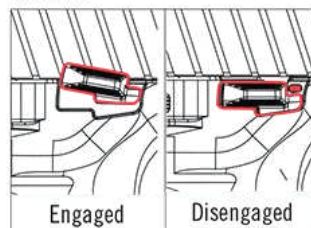
Manual safety.
