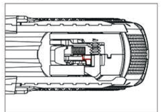
Trigger disconnect.
