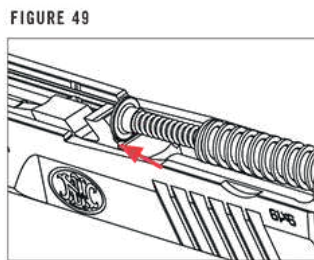
Align recoil spring.
