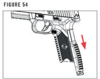
Backstrap removal.
