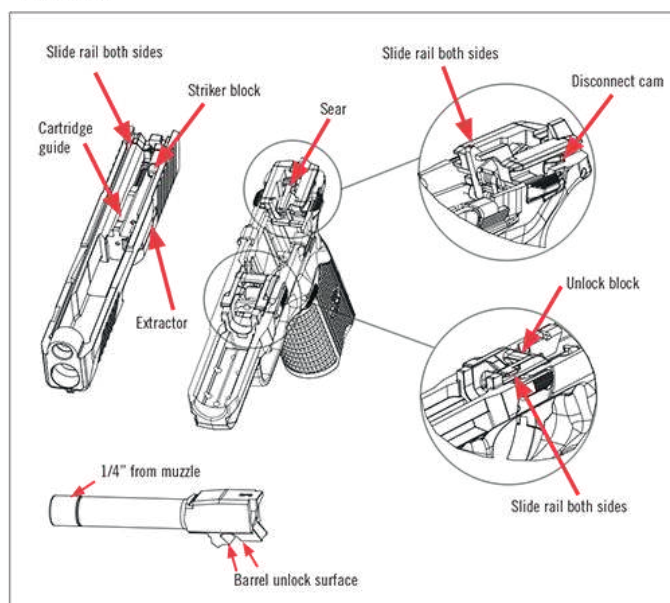
Lubrication Points.
