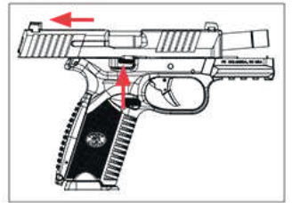
Lock slide open.
