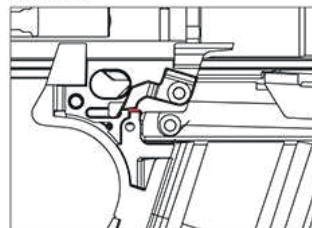
Drop safety.
